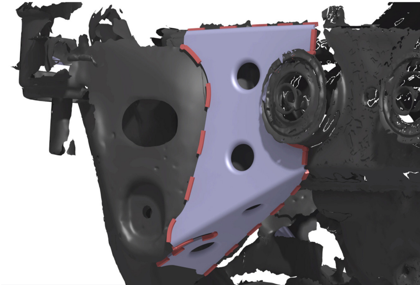
Image 3. Rear differential carrier's left side stich welding right view
