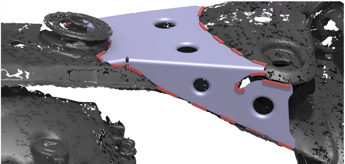
Image 7. Rear differential carrier's right side stitch welding left view
