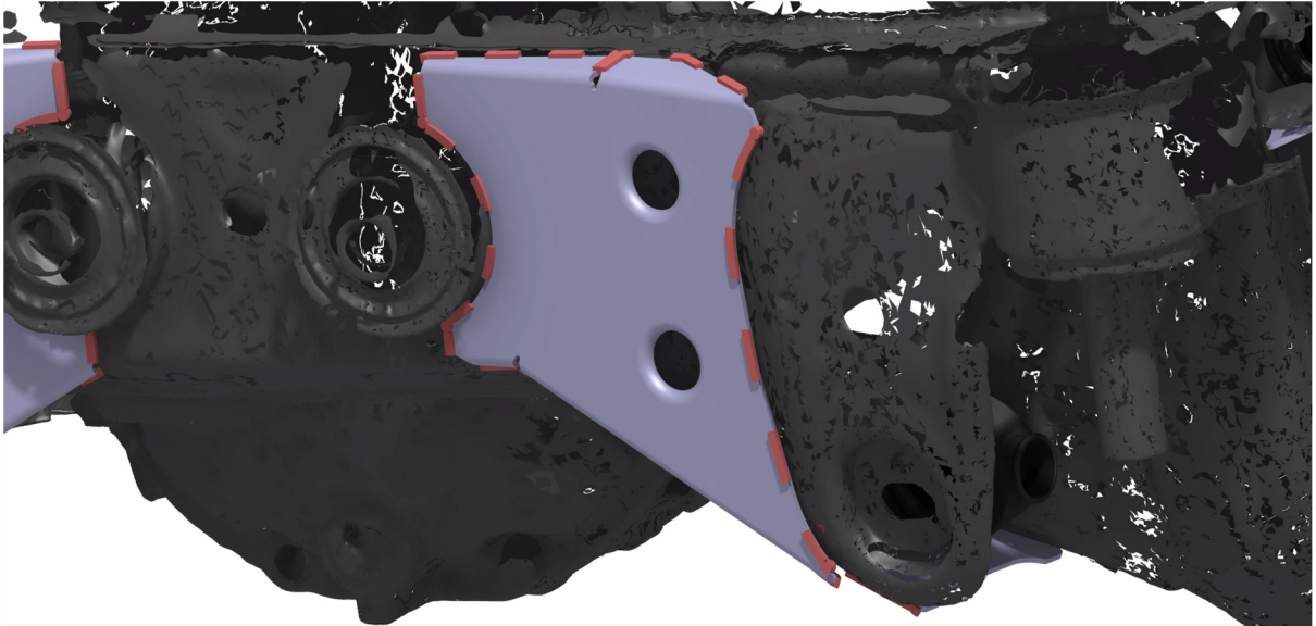
Image 6. Rear differential carrier's right side stitch welding right view
